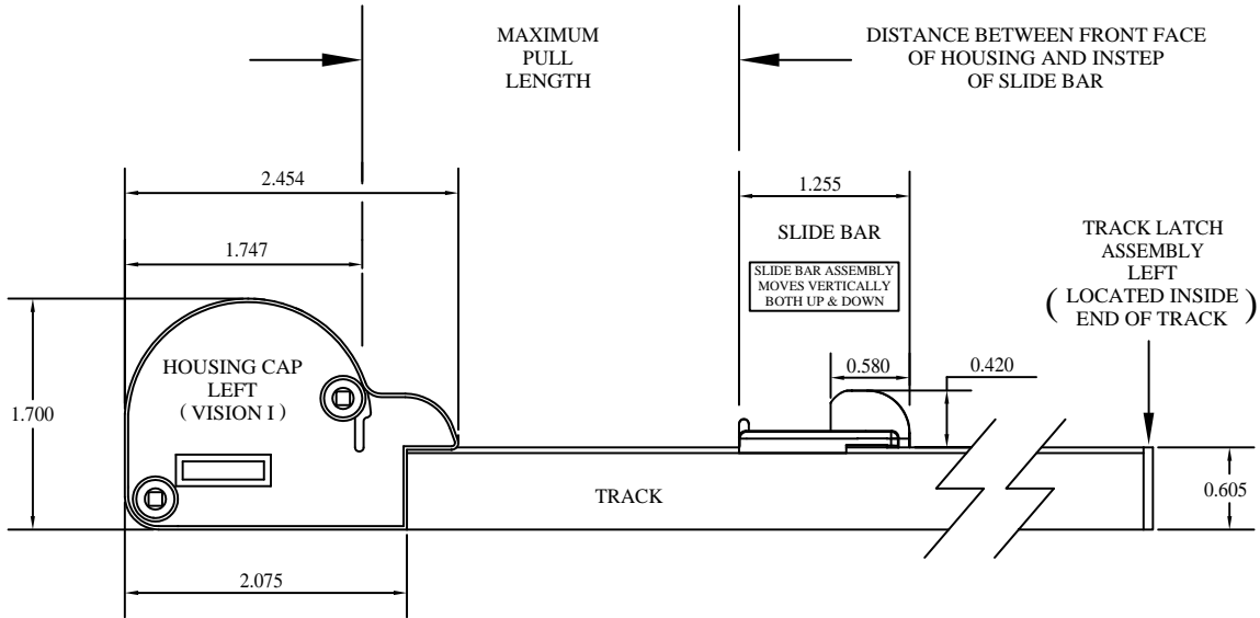
VISION I WINDOW SCREEN ASSEMBLY - LEFT SIDE VIEW
