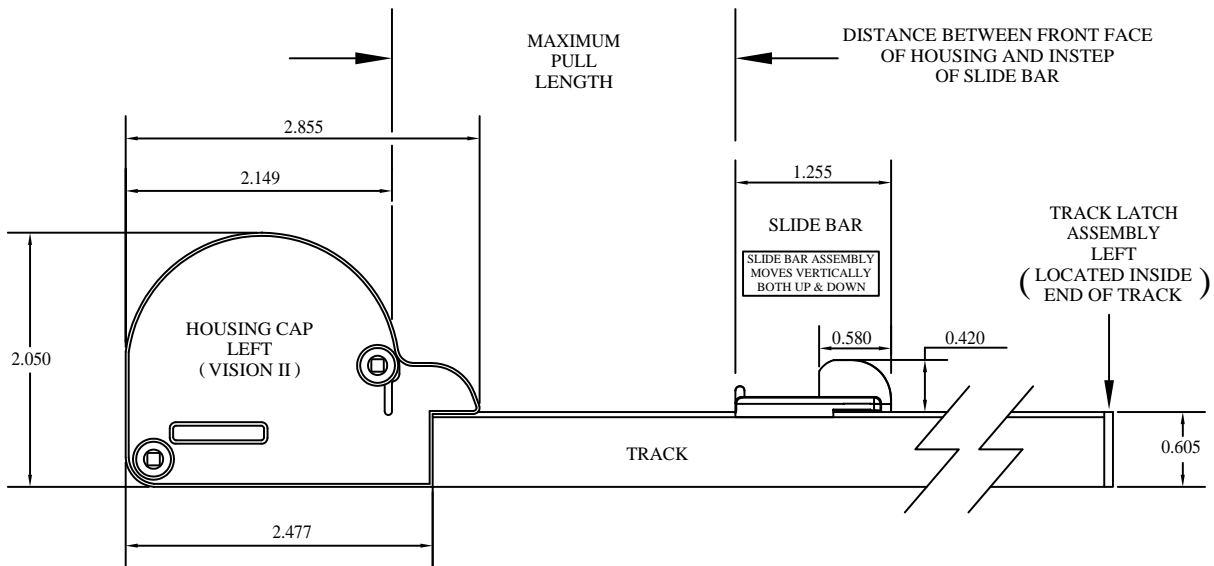
VISION II WINDOW SCREEN ASSEMBLY - LEFT SIDE VIEW
