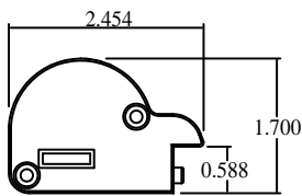
Vision I Housing End Cap Left Side View (External)
