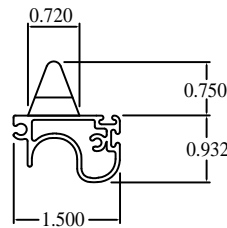
Cross Section Through Slide Bar and Handle
