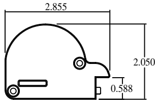
Vision II Housing End Cap Left Side View (External)
