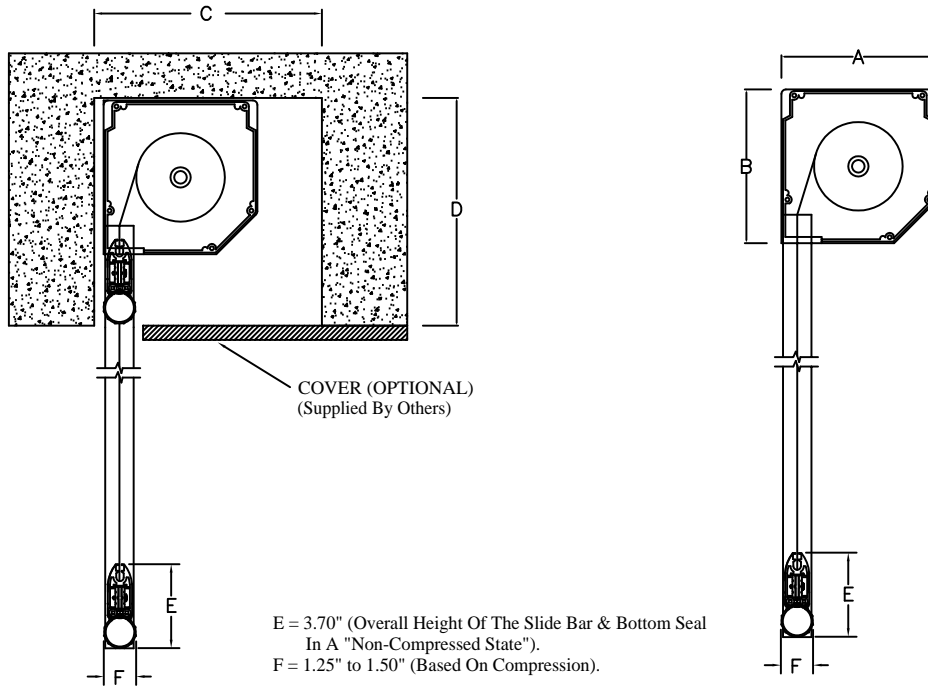
BUILT IN HOUSING ASSEMBLY INSTALLATION (CROSS-SECTIONAL VIEW)
