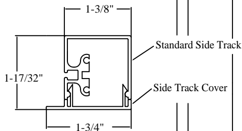
CROSS SECTIONAL VIEW OF THE STANDARD SIDE TRACK (V2)
